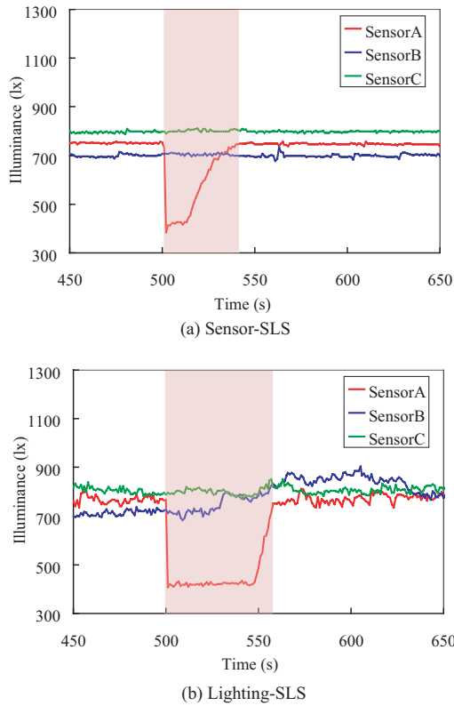
Fig. 7. Illuminance history (Experiment 2)
